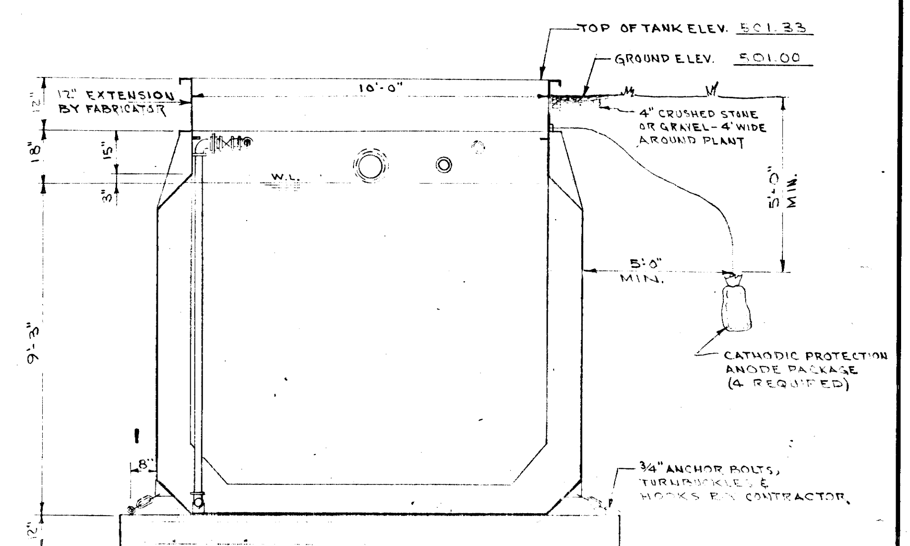
SECTION C-C
