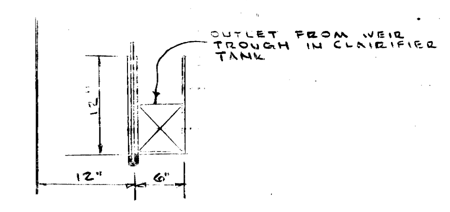
SECTION 2-2
