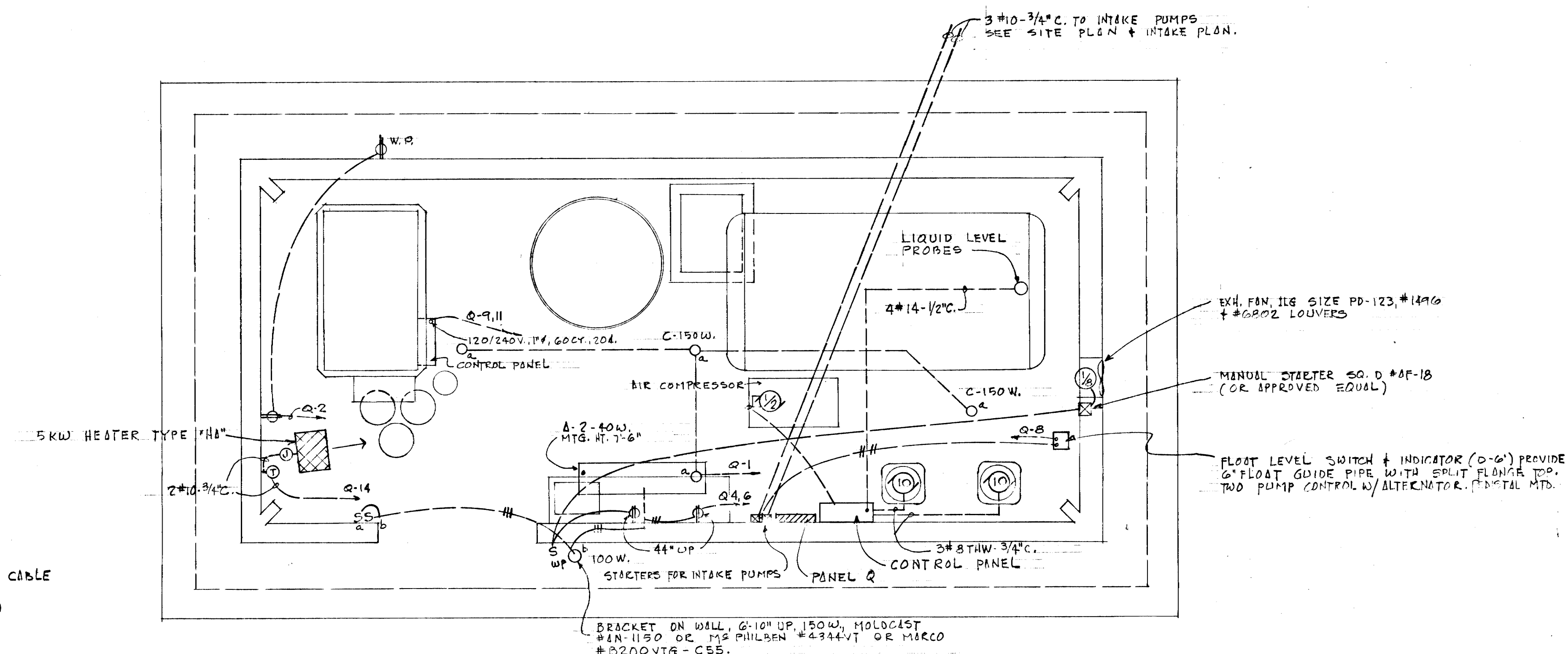
WATER TREATMENT BUILDING ELECTRICAL PLAN SCALE: 3/8" = 1'-0"
