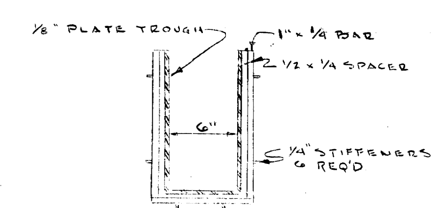
SECTION 1-1
