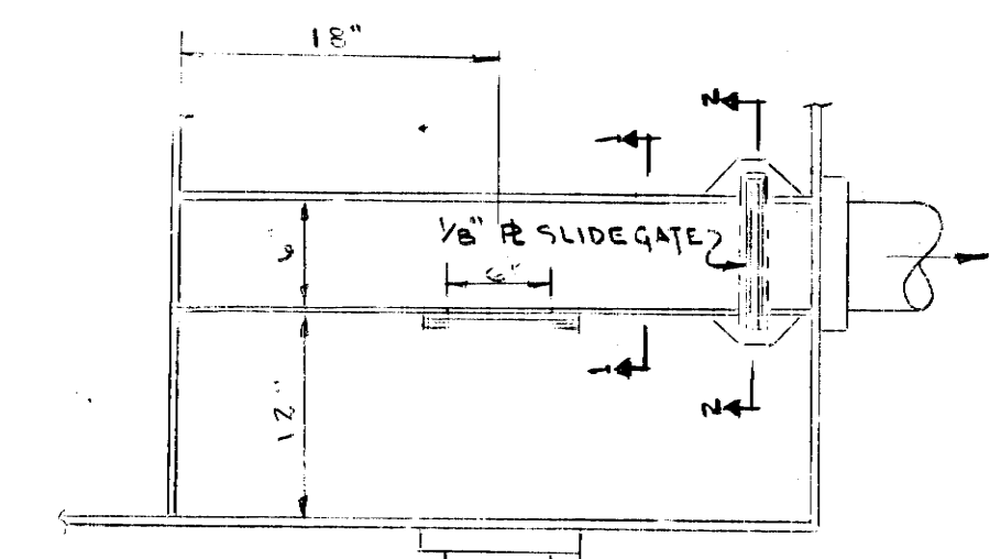
FLUME & GATE DETAIL
