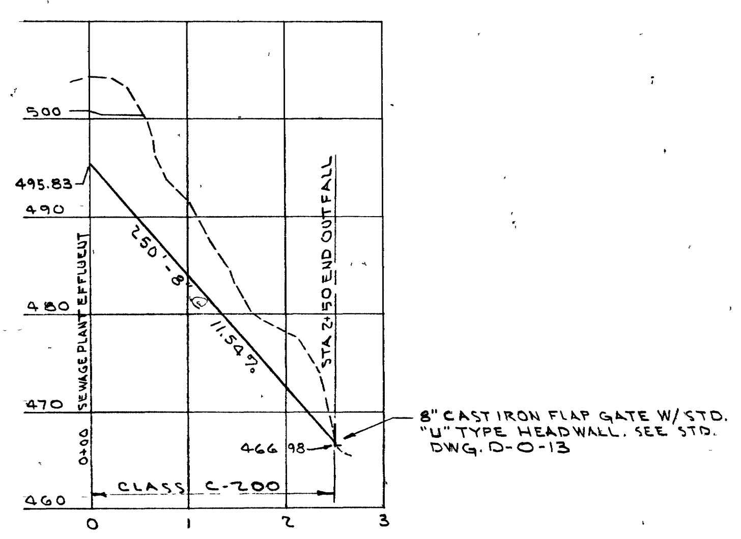
OUTFALL SEWER PROFILE
