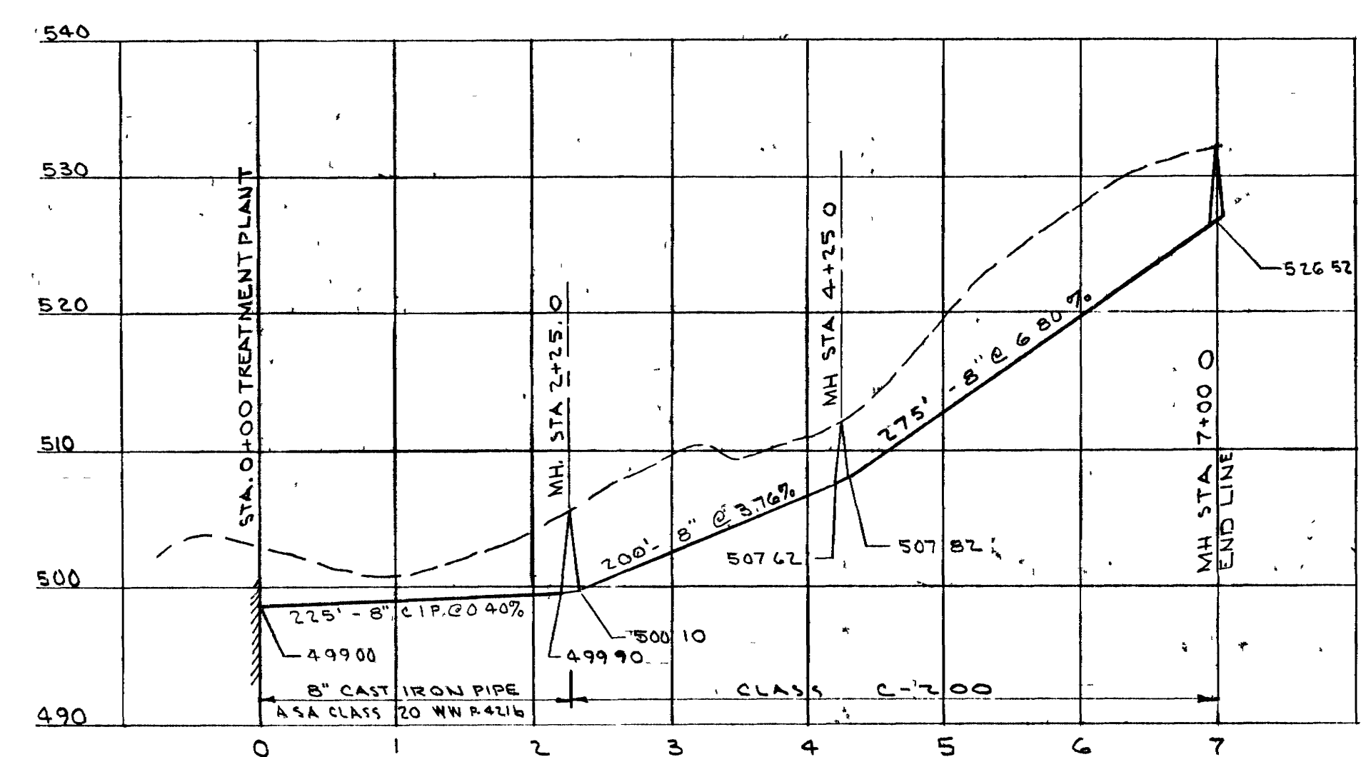
SEWER PROFILE HORIZ. SCALE 1" = 100' VERT. SCALE 1" = 10'
