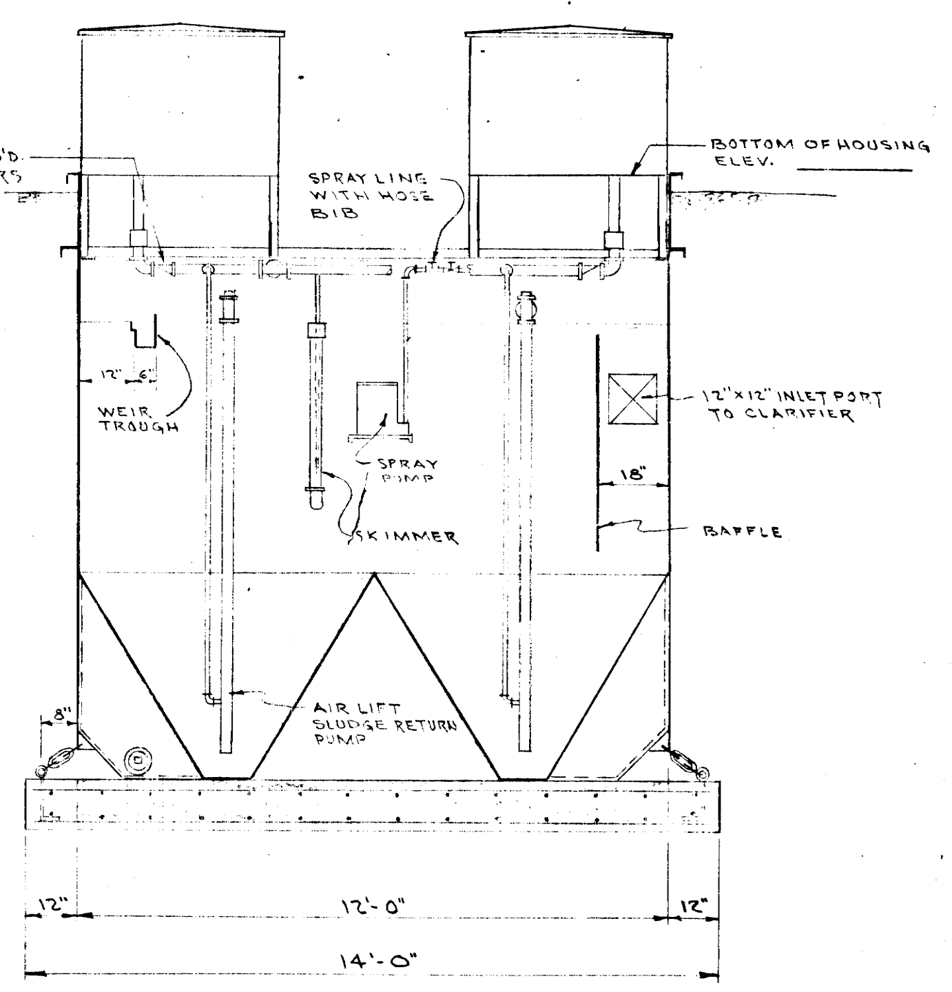
SECTION C-C
